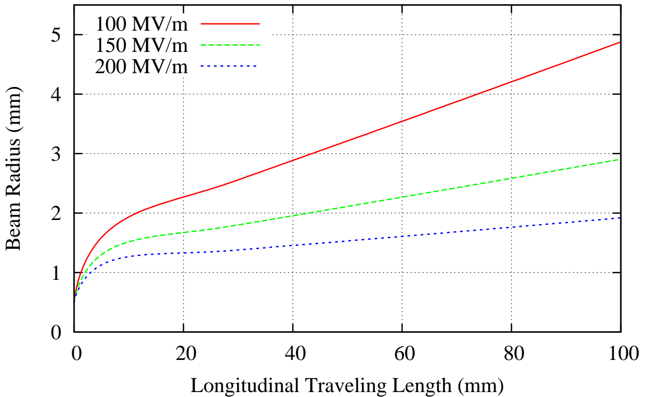
Envelop Equation with RF field Pulse width = 3mm, Beamsize = \phi 1mm, Charge = 1nC/bunch
