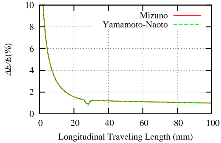
Pulse width: 3 mm, Accelerated by RF, 150MV/m
