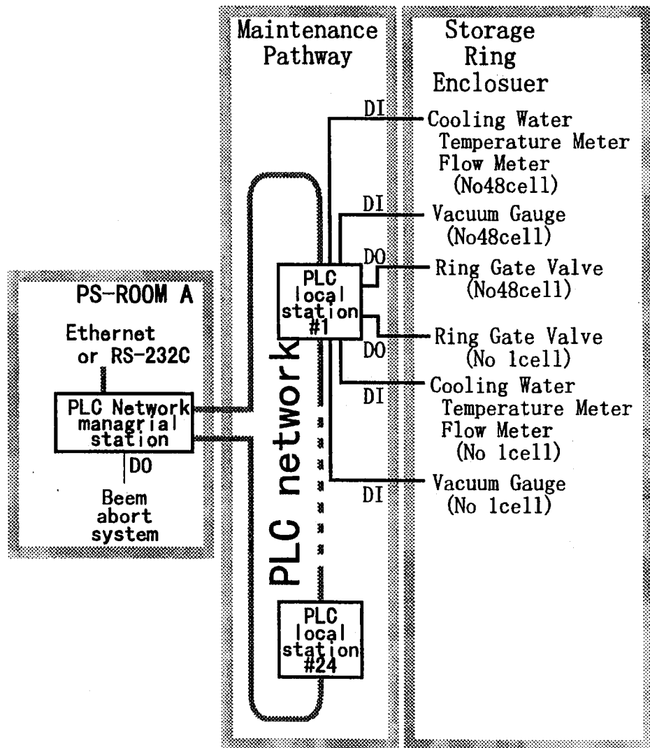
Fig.2. The abstract of PLC system
