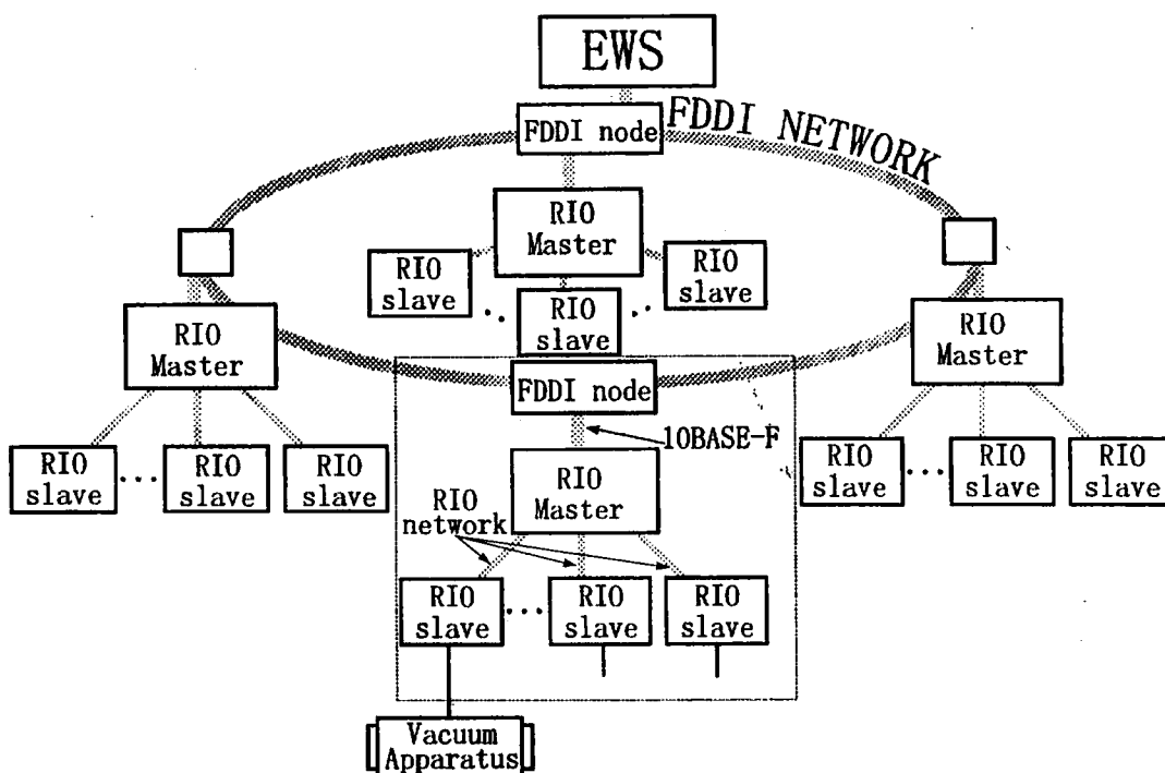
Fig.1. The abstract of VME-RIO system
