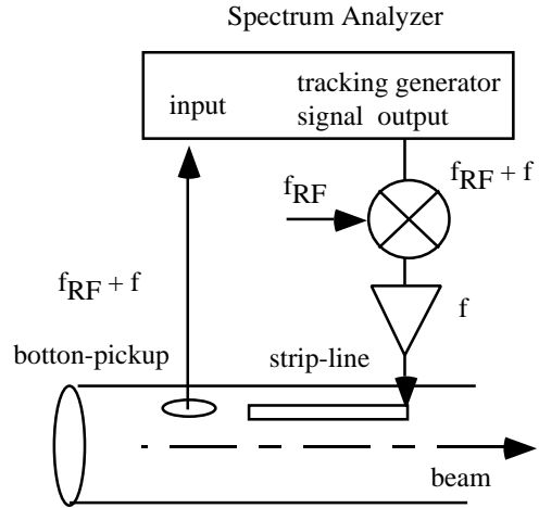
Fig. 5 Set-up for the measurement of the frequency response of the vertical betatron motion of the beam.
