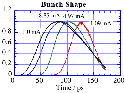
Fig.3 Bunch shape and forward shift of bunch position. As the bunch current increases, the bunch has longer tail and the timing of bunch become earlier to compensate the parasitic energy loss of the bunch. The parasitic loss is the energy radiated to wake fields at impedance.
