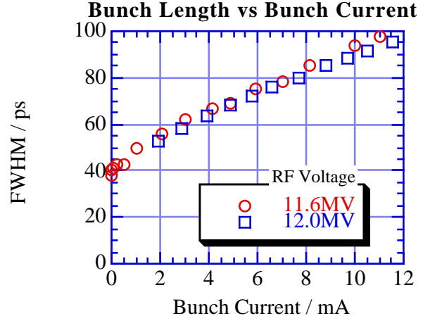
Fig.1 Bunch length vs. bunch current at two values of the RF acceleration voltages.
