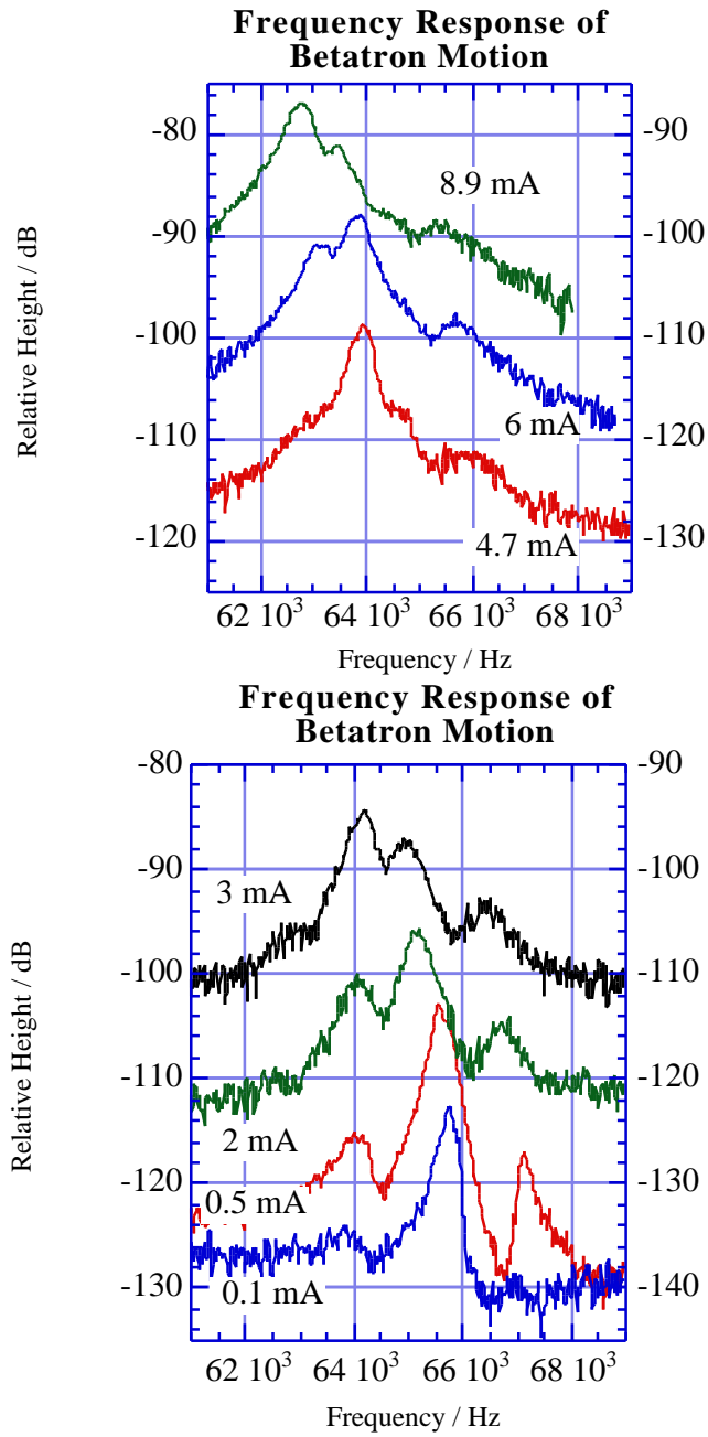
Fig. 6 Frequency response of vertical betatron motion vs. bunch current.
