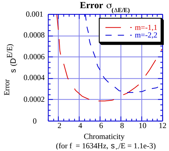
Fig. 9. Estimated error of the measured energy spread using the ratio of peak height, measured by reading error from data as video images of the spectrum analyzer display recorded as video images. This figure shows that the error is smallest at chromaticity 4 to 8.
