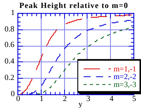
Fig. 3. Calculated ratio of peak height of m= \pm 1, \pm 2, \pm 3 to the amplitude of the peak of m=0 . y = x s_d / \eta_s .
