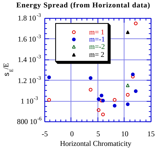
Fig. 6. The energy spread of the beam obtained from the ratio of chromatic sideband peak height relative to m=0 main peak for horizontal betatron motion. From Fig. 3, the error is smallest at chromaticity \sim 4-8 for m=\pm 1 peaks and \sim 8 for m=\pm 2 peaks as shown in Fig. 3.
