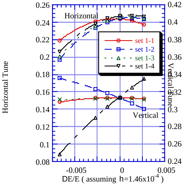
Fig. 5 Energy dependence of the betatron tune( m=0 ) assuming the momentum compaction factor is
