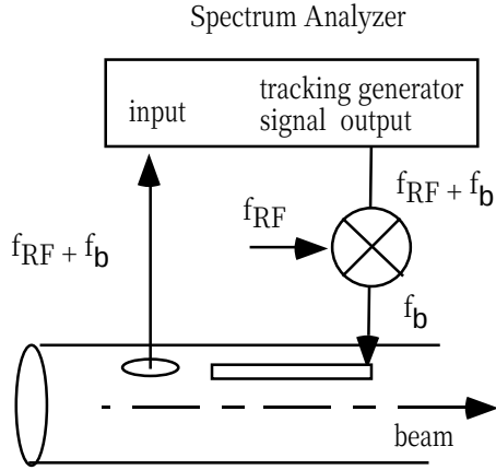
Fig. 4. Setup for measurement of frequency response of betatron motion of the beam in the storage ring. A spectrum analyzer generated the signal of frequency f = f_{RF} + f_b , where f_{RF} is RF frequency and f_b is the betatron frequency, and this signal was down-converted by a double-balanced mixer to the frequency f_b to shake the beam. The transverse motion of the beam excited by this signal is detected by a button-type pick-up electrode at frequency f = f_{RF} + f_b .
