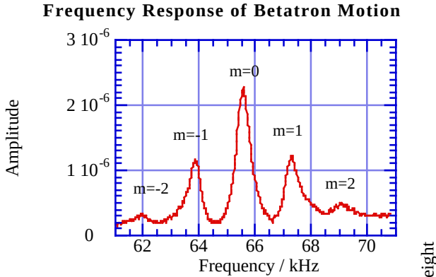
Fig. 1. Typical data of the frequency response of the betatron motion of the beam in the SPring-8 storage ring. The direction of betatron motion is vertical and the vertical chromaticity is 8.8 ( y \sim 1 ) and the height of the m=0 peak is reduced to be a half of that at chromaticity 0 as shown in Fig. 2. The mode number m of each peak is also shown. This signal was averaged during 10 sweeps.
