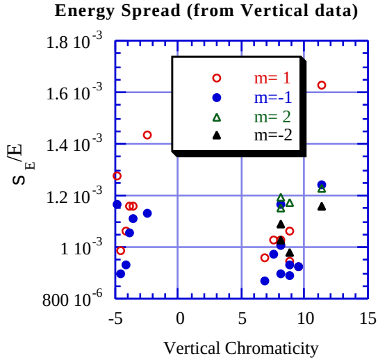
Fig. 7. The energy spread of the beam obtained from the ratio of chromatic sideband peak height relative to m=0 main peak for vertical betatron motion.
