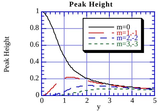
Fig. 2. Calculated relative peak height for m=0, \pm 1, \pm 2, \pm 3 based on Ref.[1]. y = x s_d / \eta_s
